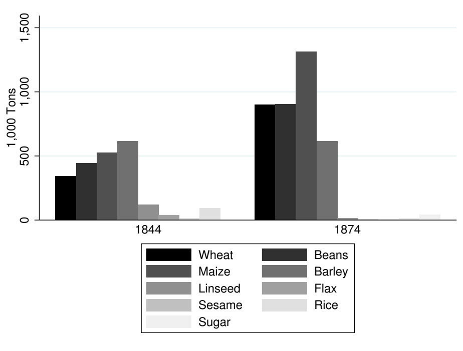
Figure A.5 – Total output of major export crops (except cotton and cotton seed) in Egypt in 1844 and 1874
